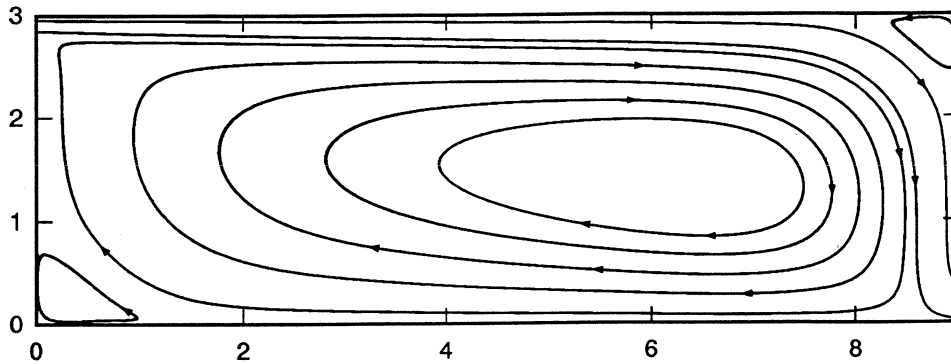
b. Flow field in the ventilation enclosure
