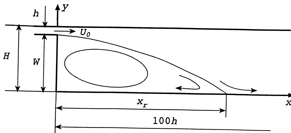
Figure 1. Backward-facing step configuration.
