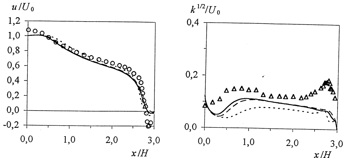
Figure 6. Distributions calculated with the wall-function method. — — — SKE,
