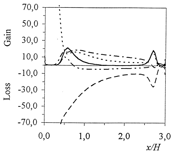
Modified \omega -equation.
