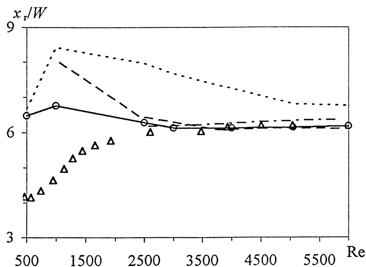
Figure 2. Reattachment length versus Reynolds number, x_r/W \sim Re .
