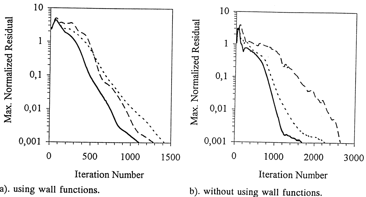
Figure 10. Comparison of the convergence procedure with various models. --- SKE or LBKE, ..... WKW, _____ Present.
