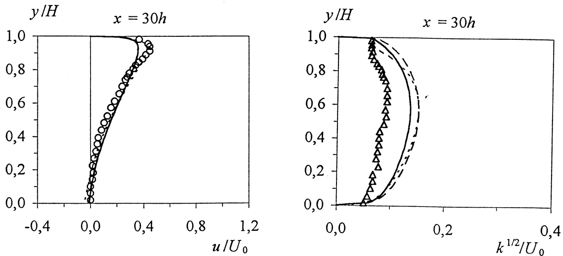
Figure 3. Distributions calculated with the wall-function method. — — — SKE, ..... WKW, ——— Present. \Delta Measured \sqrt{u'^2}/U_0 , \circ Measured u/U_0 .
