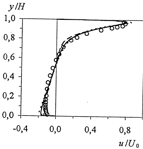
Profiles at vertical cross section x = H .
