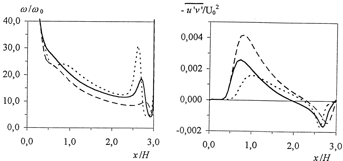
Profiles at horizontal cross section y = H - h/2 .
