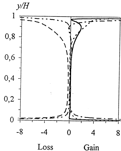
Modified \omega -equation.
