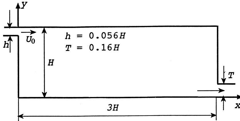
a. Geometry of the ventilation enclosure.
