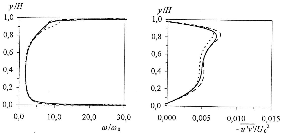
Profiles at vertical cross section x = 2H .
